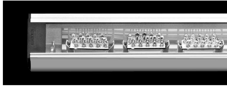
Photo : LL3AL IP65 with AGA-LED® A-10 lighting units rigid loop connector / 24V / 1W
