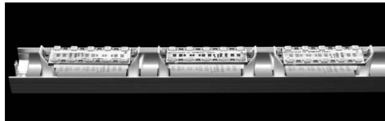
Photo: LU4AL IP20 with AGA-LED® B-10 lighting units rigid loop connector / 24V / 1W
